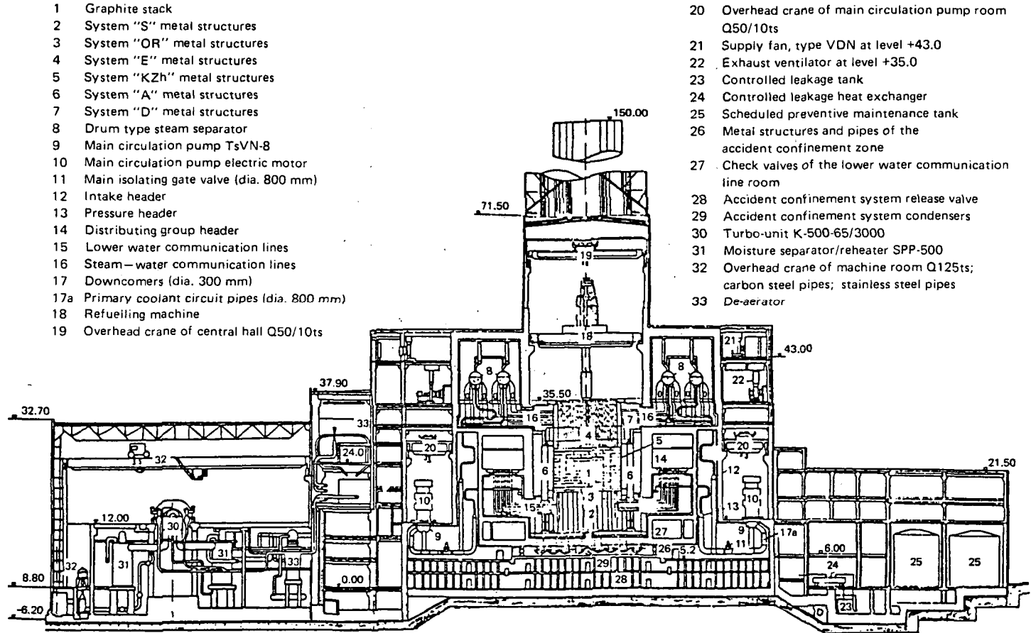
FIG. 6. Vertical section showing the principal installations in the main block of Chernobyl Unit 4. Dimensions are in metres.
