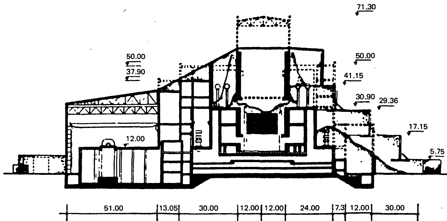
FIG. 4. Vertical section of the projected entombment structure for Chernobyl Unit 4. Dimensions are in metres.
