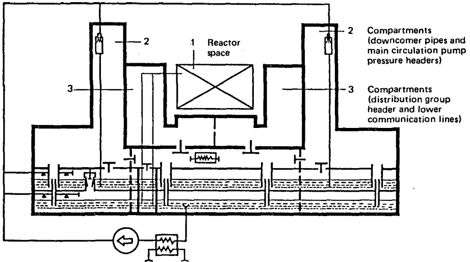
FIG. 12. Schematic diagram of part of the containment system (the 'accident localization system').
