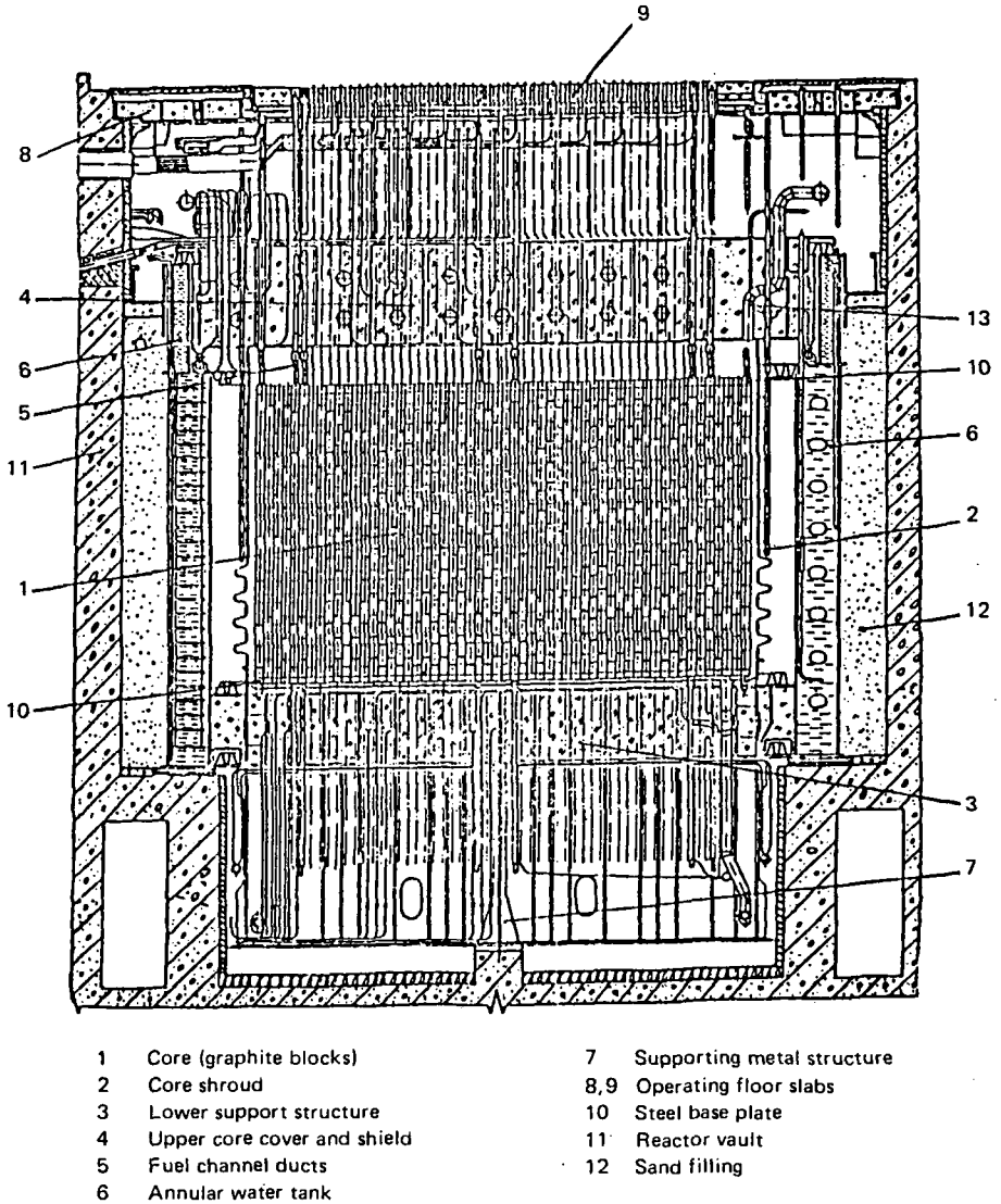
FIG. 8. The arrangement of the core of Chernobyl Unit 4.
