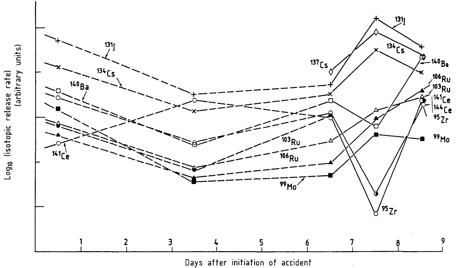
FIG. 3. Isotopic release rates derived from data provided in the Soviet Working Documents. Note that these data are preliminary and may not be representative of all the data collected by the Soviet experts.
