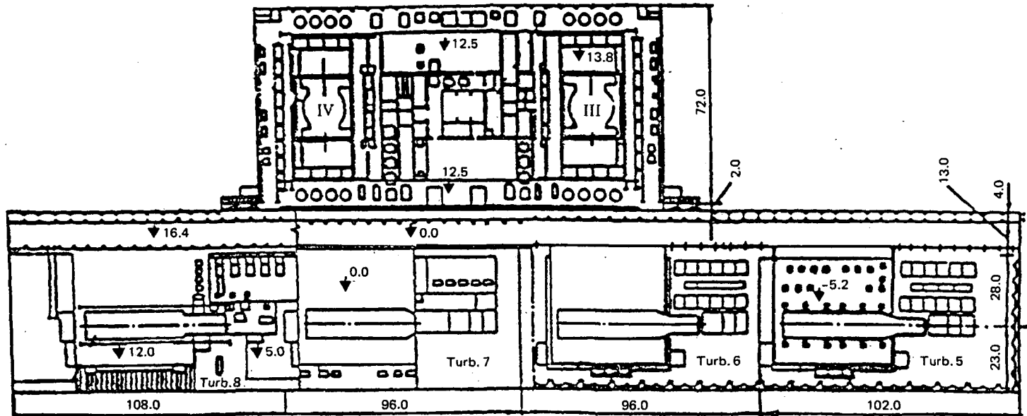
FIG. 7. Plan of the main building of Chernobyl Units 3 and 4. Dimensions are in metres.
