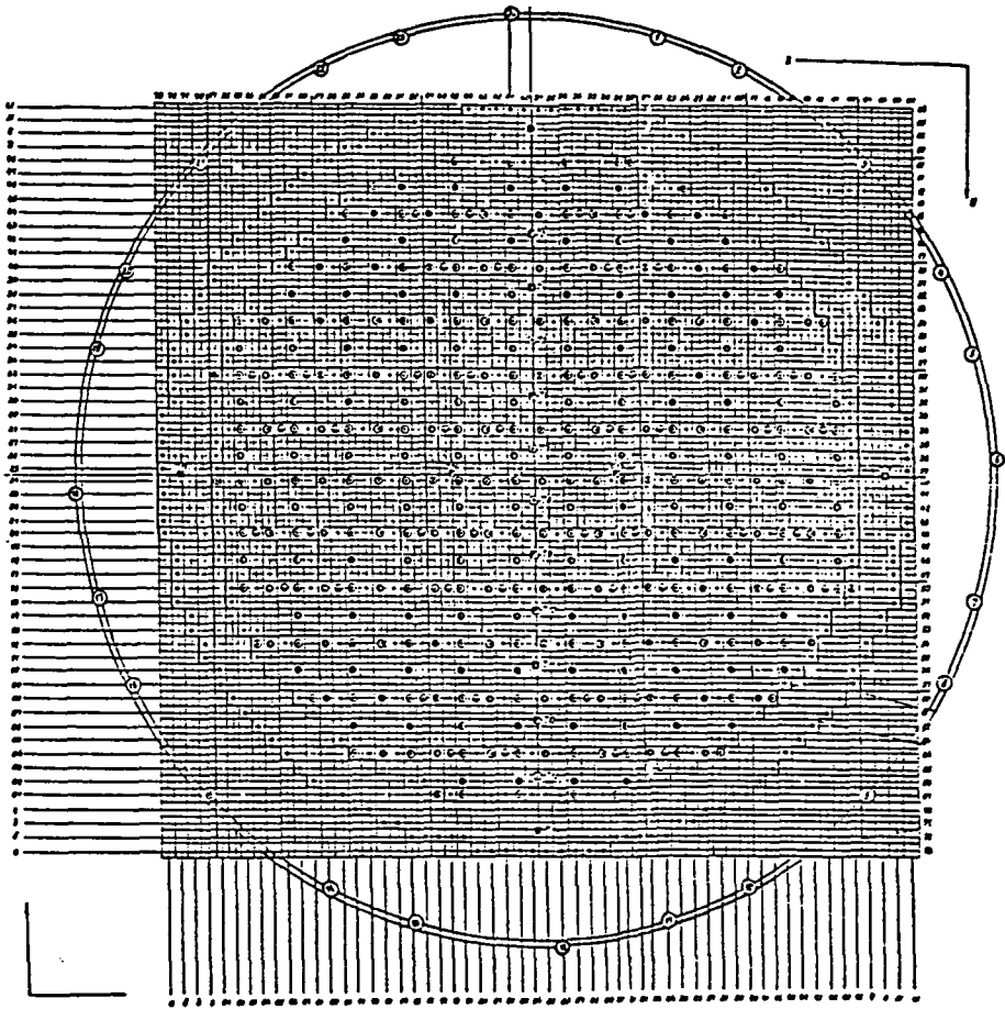
FIG. 10. Horizontal section of the core of the Chernobyl Unit 4 reactor showing the positions of the control rods.
