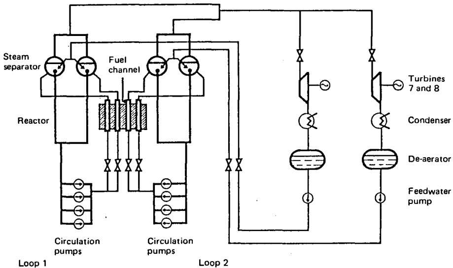
FIG. 9. Schematic diagram of the main water and steam circuits of Chernobyl Unit 4.
