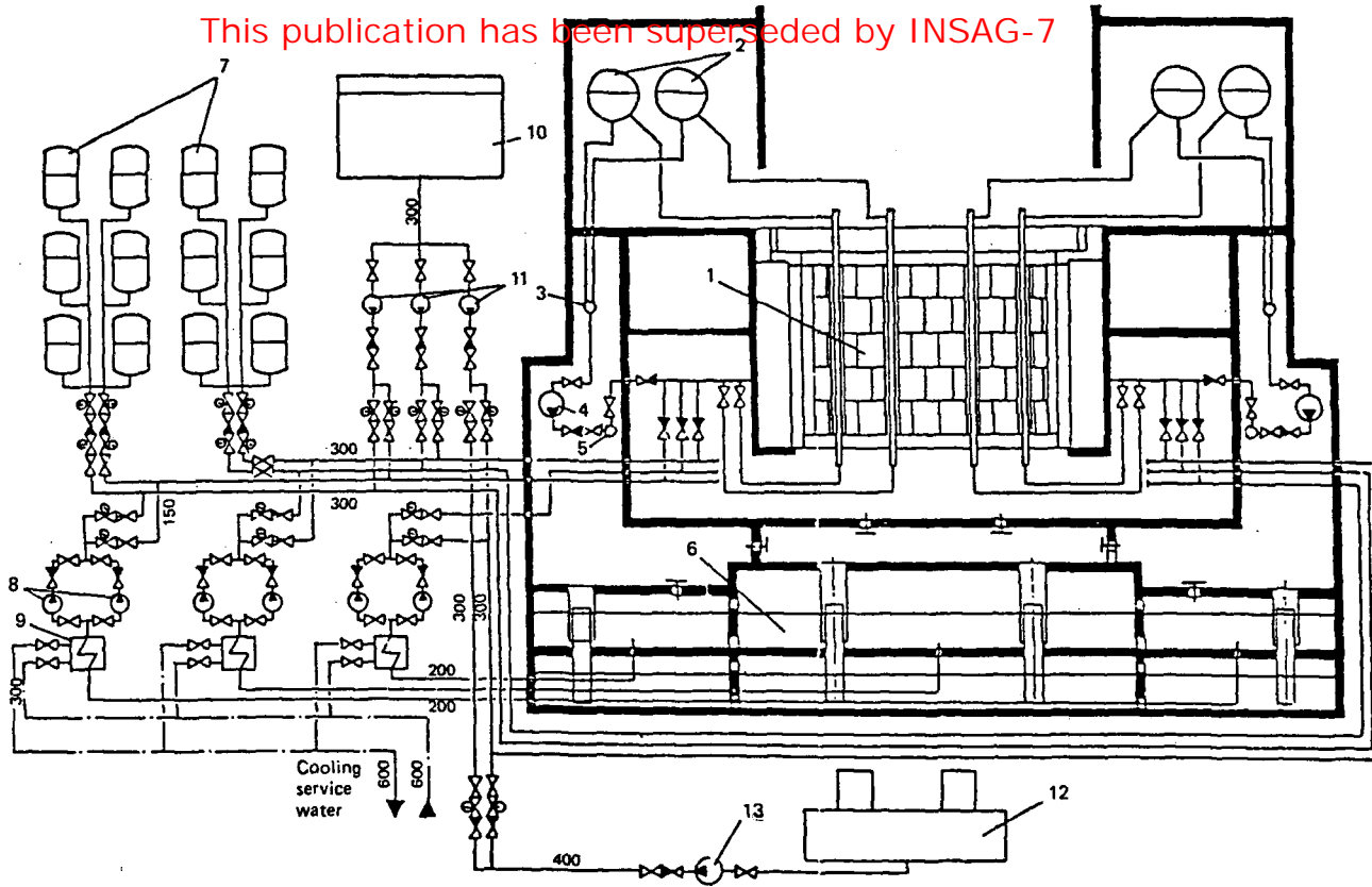
FIG. 11. Schematic diagram of the emergency core cooling system (ECCS) of Chernobyl Unit 4. Key: 1: reactor; 2: steam separators; 3: suction header; 4: main circulation pump; 5: pressure header; 6: pressure suppression pool; 7: ECCS vessels; 8: ECCS pumps for cooling the damaged half of the reactor; 9: heat exchangers; 10: clean condensate container; 11: ECCS pumps for cooling the undamaged half of the reactor; 12: de-aerator; 13: feed pump.
